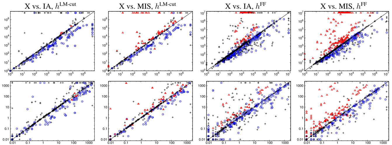
Figure 3: Scatter plots, with a data point per instance, showing the search space size (top), and runtime in seconds (bottom) of X vs. IA/MIS, with X on the x-axis and IA/MIS on the y-axis. Black points indicate instances where both strategies did not abstain. Blue circles (red triangles) highlight instances for which X (IA/MIS) has abstained; we show data for B in this case.
