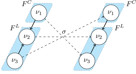
Figure 1: A structural symmetry \sigma that is not a decoupled symmetry for the depicted factoring.
