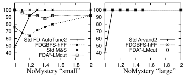
Figure 5: % instances covered in Nakhost et al.’s (2012) NoMystery test suites, over resource constrainedness (factor by which the available fuel exceeds the minimum required).
